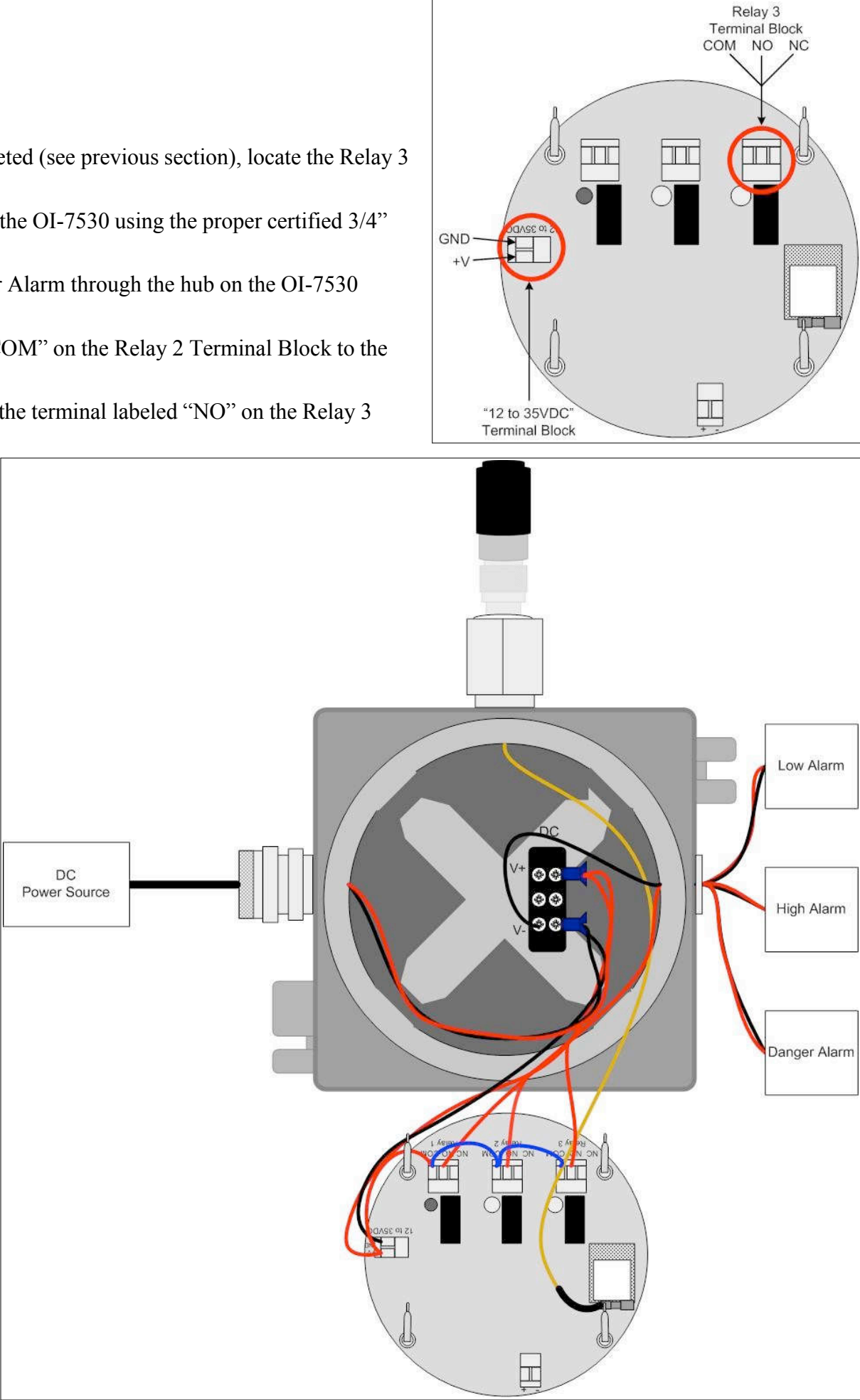
DC Wiring Configurations - Complete Wiring Diagram (power and all three relays connected)
