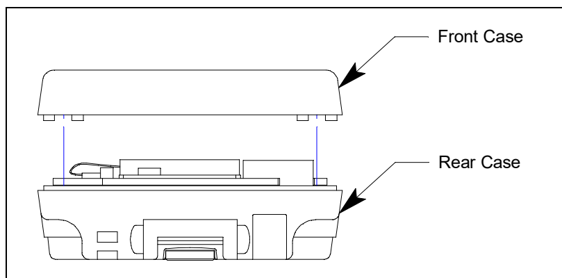
Figure 15: Case Separation
