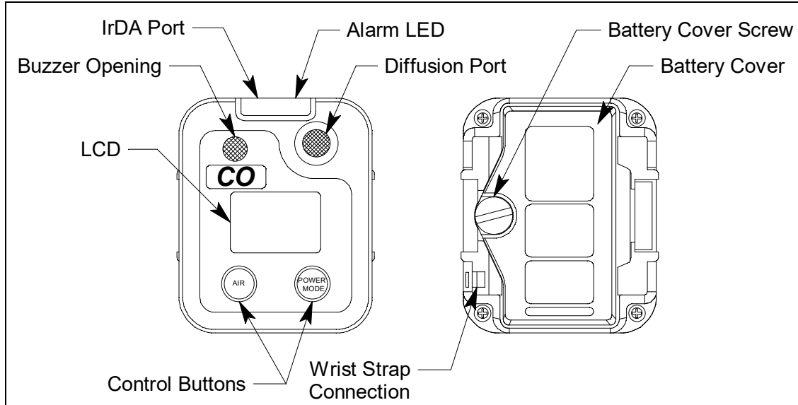
Figure 1: Component Location
