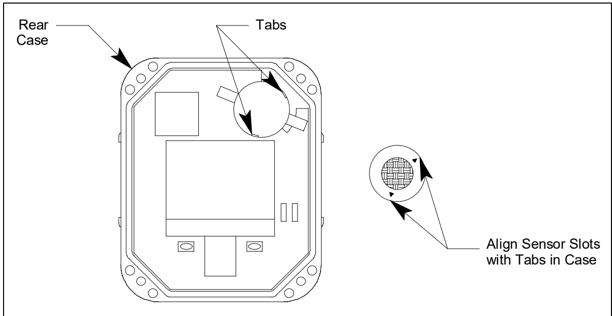
Figure 16: Sensor Location
