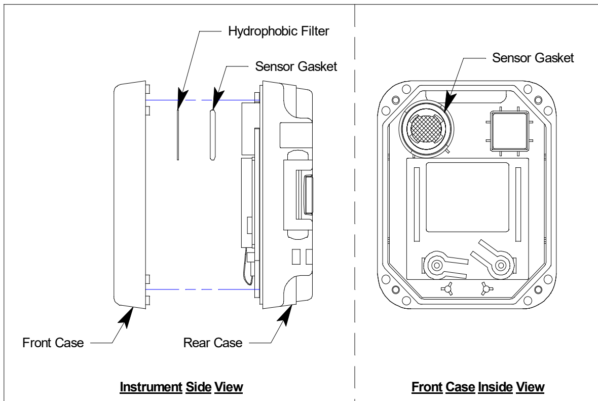
Figure 13: Hydrophobic Filter Location
