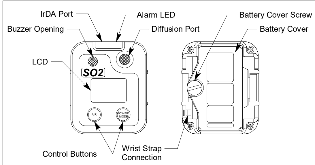
Figure 1: Component Location
